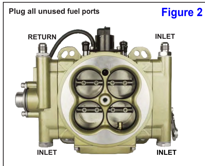
The FiTech Go EFI Throttle Body has (3) Inlet Ports and (1) Return Port. The Return Port is plugged when using the Force Fuel Mini.
