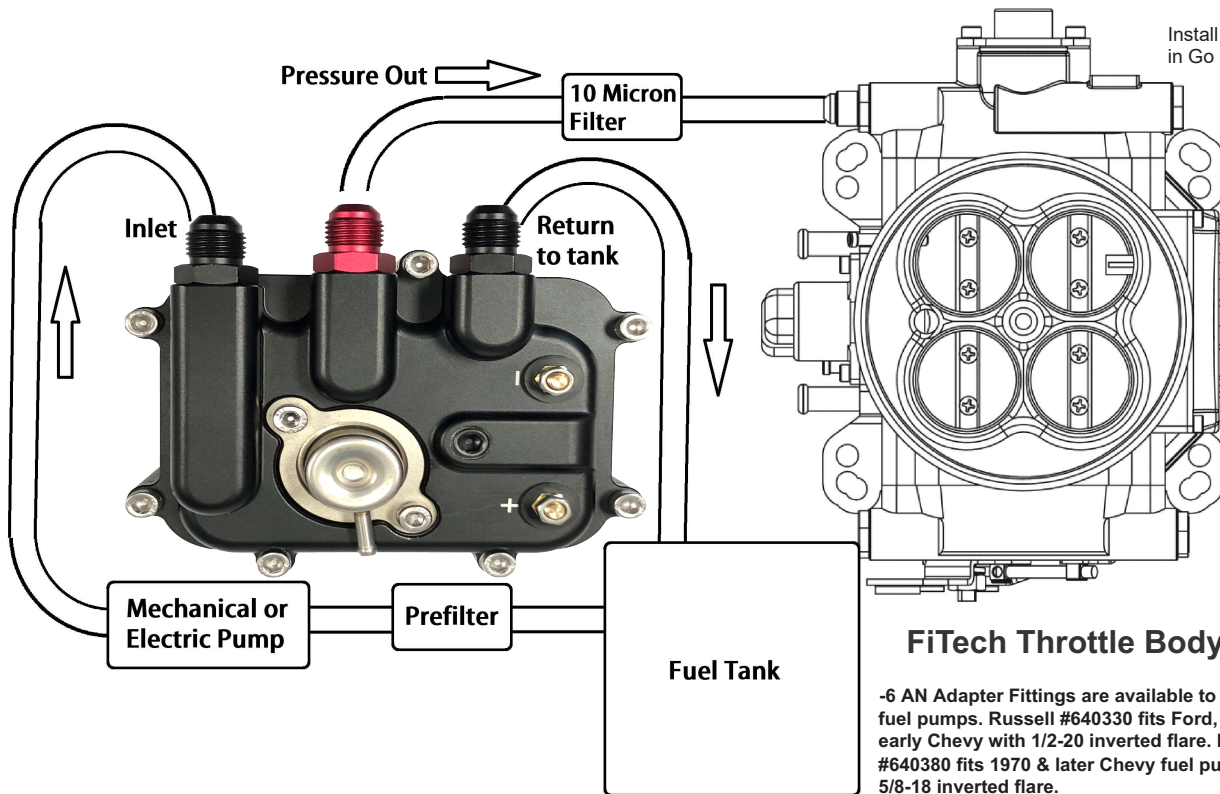
Plumbing Schematic for FiTech Force Fuel Mini - Fuel Delivery Kit #50006
